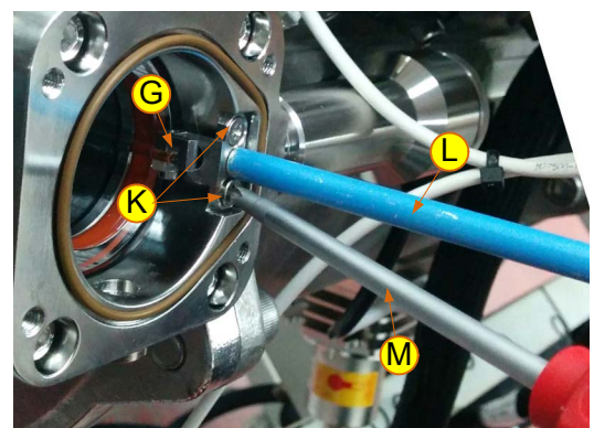
Figure 10-21: Unfastening the Wave Guide (Generic View)
