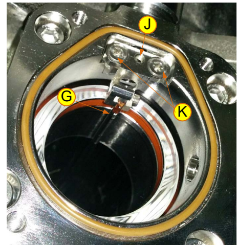
Figure 10-19: Wave Guide Elements (Generic View)
