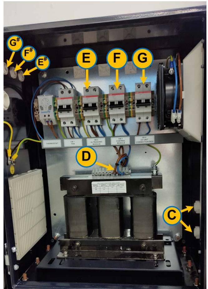
Figure 5-34: Power Module - connections
