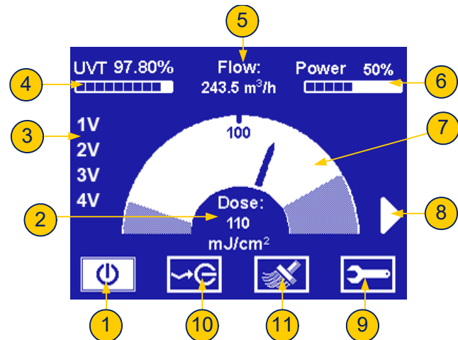
Figure 6-1: Initial Main Operation Screen
