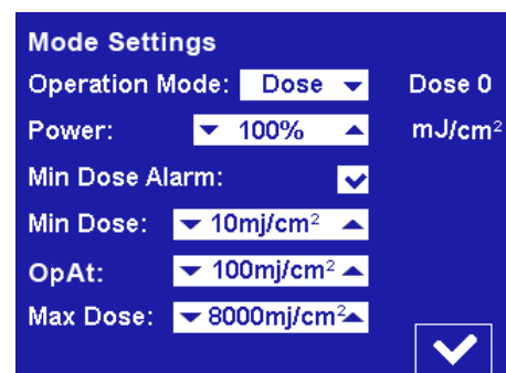
Figure 6-4: Dose Settings Screen
