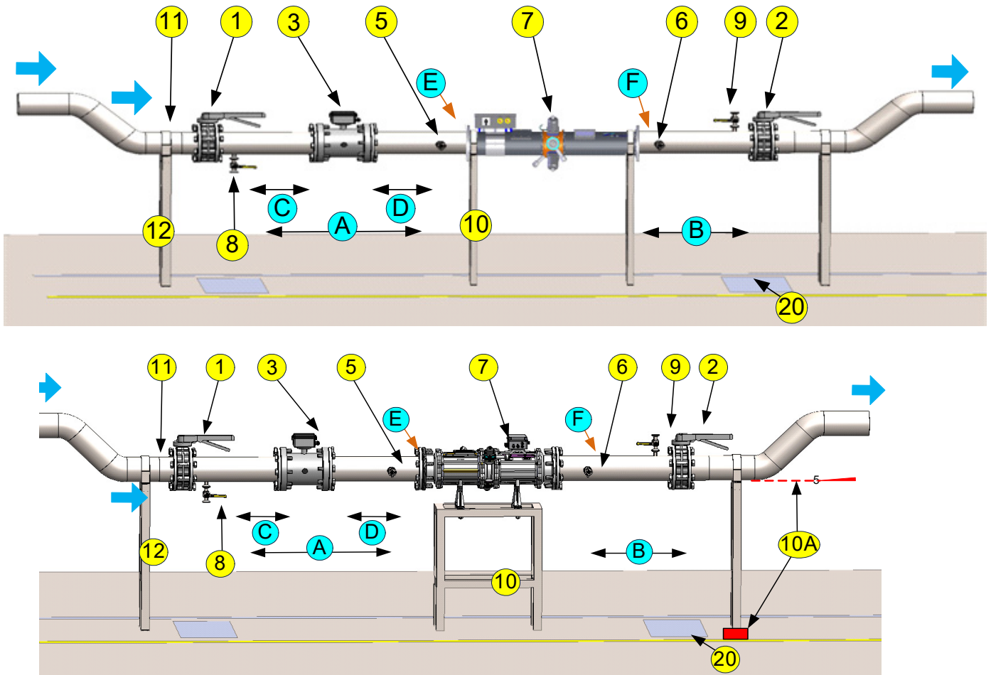
Figure 3-1: Generalized Atlantium system setup, horizontal (no bypass)
