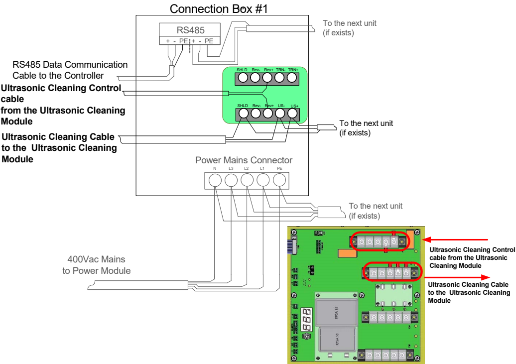
Figure 5-30: Cabling Schematic Diagram
