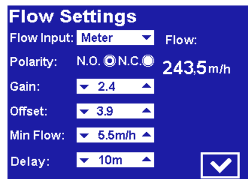
Figure 8-1: Flow Settings Screen
