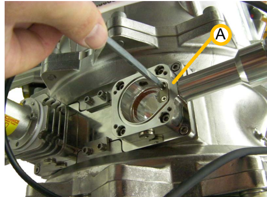
Figure 10-23: (Generic) Cleaning the UV Intensity Sensor's Mirror
