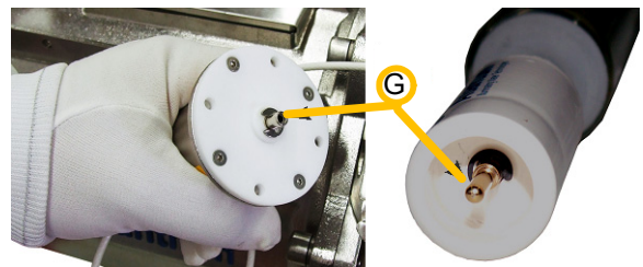
Figure 10-16: Lamp, Connector Assembly and connectors
