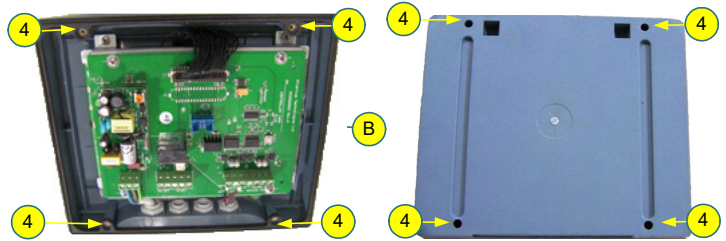
Figure 5-23: Control Module's Circuit Board
