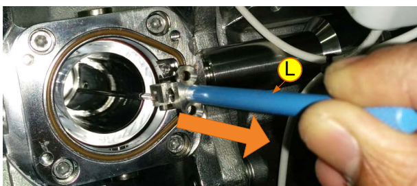
Figure 10-20: Removing the Wave Guide (Generic View)
