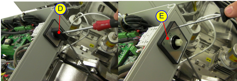
Figure 5-37: Replacing the Power Cable 1
