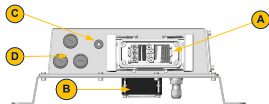
Figure 5-26: Ballast Module C-Waterproof Box (bottom view)
