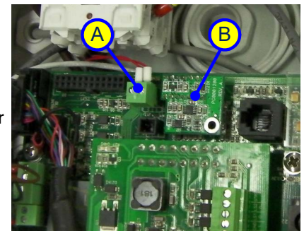
Figure 10-42: Location of the Temperature Sensor Connector (Generic)
