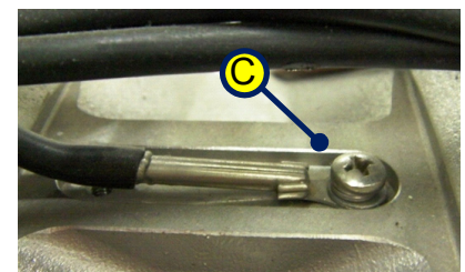
Figure 10-43: Location of the Temperature Sensor on the Atlantium Unit
