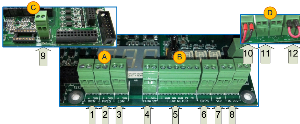
Figure 5-35: Connectors on Connection Box Card 1300+1400
