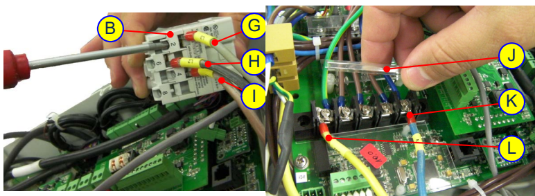
Figure 5-40: Replacing the Power Cable 4
