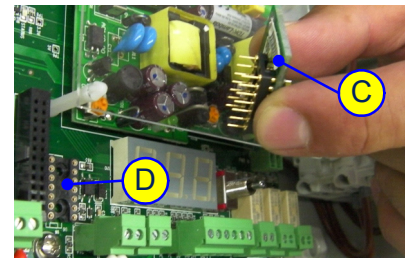
Figure 10-44: Replacing the Temperature Sensor Card (Generic)
